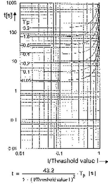
Figure 12-1 Operate Curves and Dropout Time Characteristic Curves According to IEC
