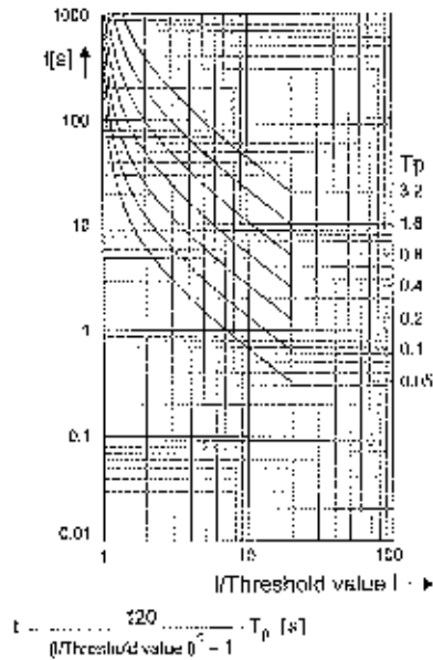
Figure 12-2 Operate Curves and Dropout-Time Characteristic Curves According to IFC
