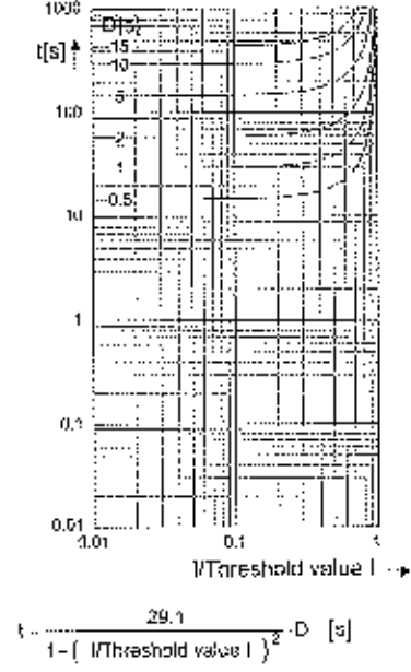
Figure 12-11 Operate Curves and Dropout-Time Characteristic Curves According to ANSI/IEEE
