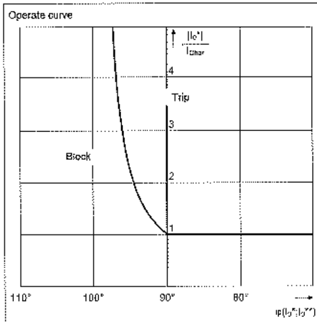
Figure 12-20 Restricted Ground-Fault Protection Operate Curve depending on the Phase Angle between I_a^* and I_b^{**} at |I_a^*| = |I_b^{**}| (180° ~ External fault)
