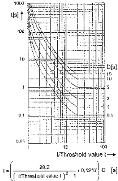
Figure 12-11 Operate Curves and Dropout-Time Characteristic Curves According to ANSI/IEEE
