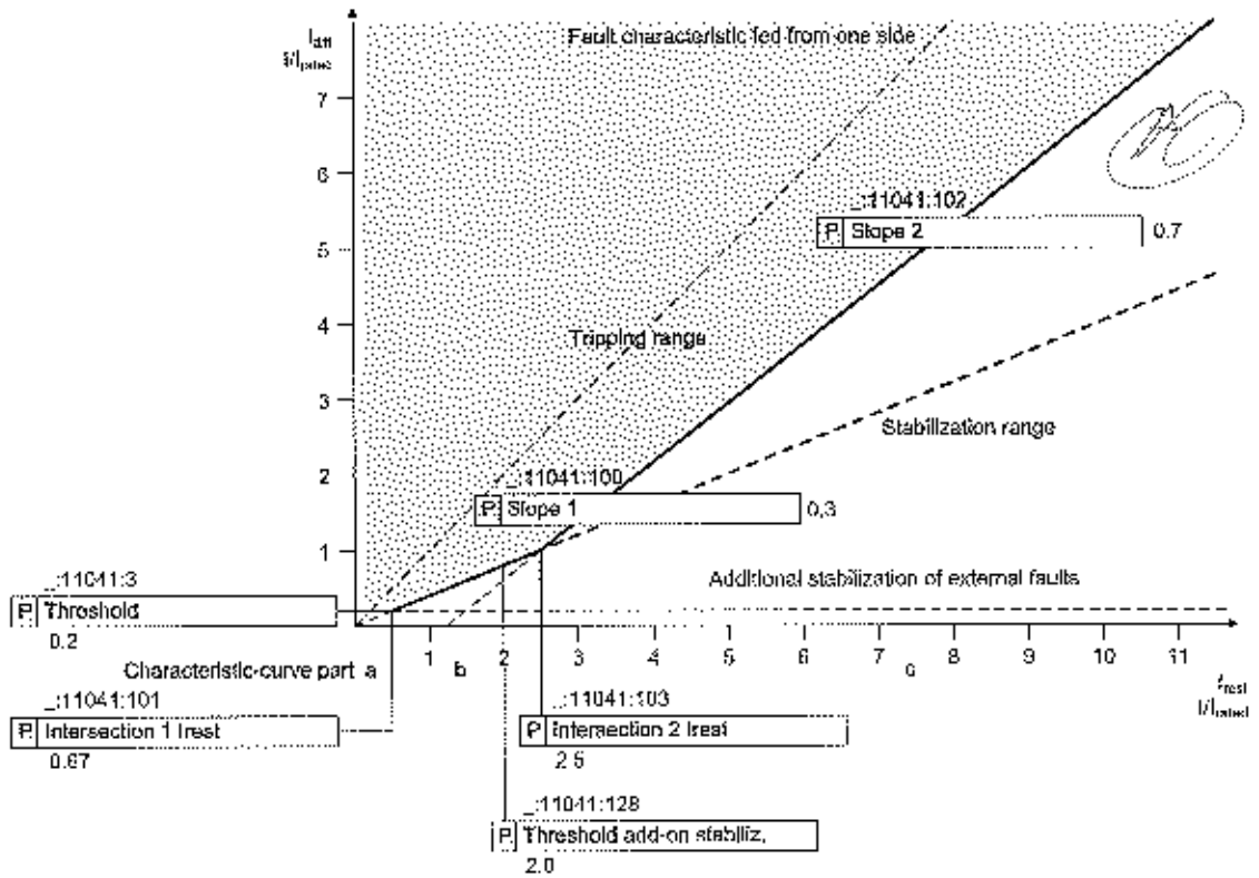
Figure 12-17 Operate Curve of the Differential Protection
