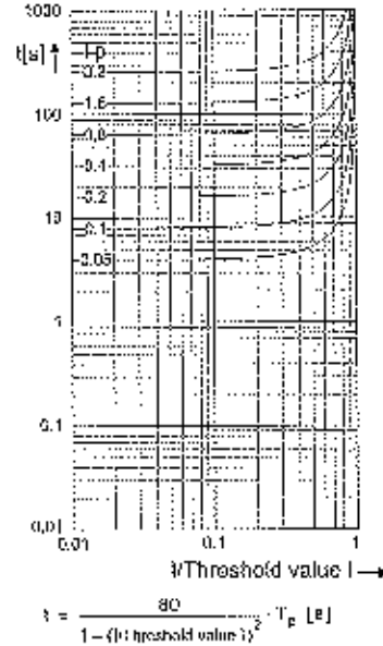
Figure 12-2 Operate Curves and Dropout-Time Characteristic Curves According to IFC
