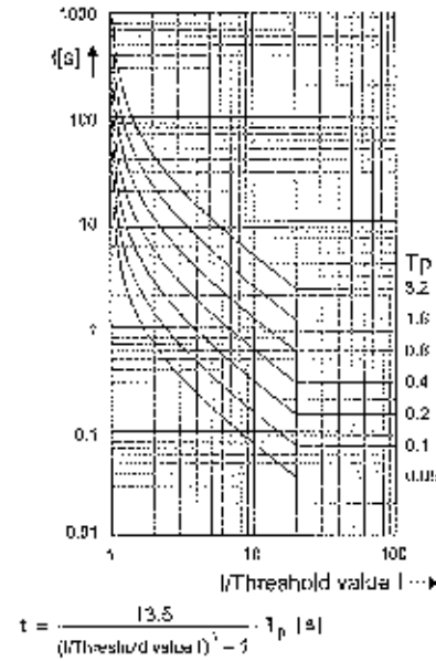
Figure 12-1 Operate Curves and Dropout Time Characteristic Curves According to IEC
