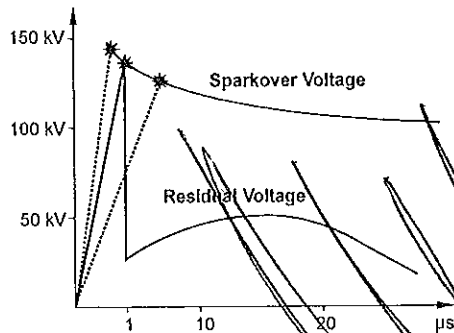
20 kV System
