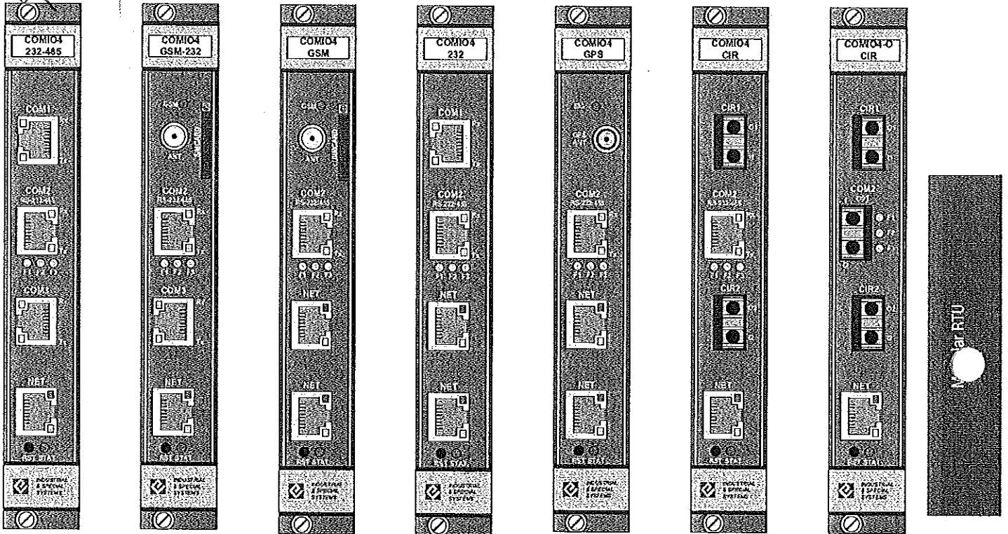
Front panels with connectors of cards COMIO4
