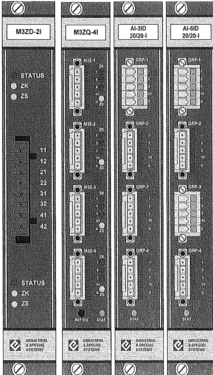
Рис. 54 - RTU7M-M3ZD-2I, RTU7M-M3ZQ-4I, RTU7M-AI-3ID/20/20-I, RTU7M-AI-6ID/20/20-I
