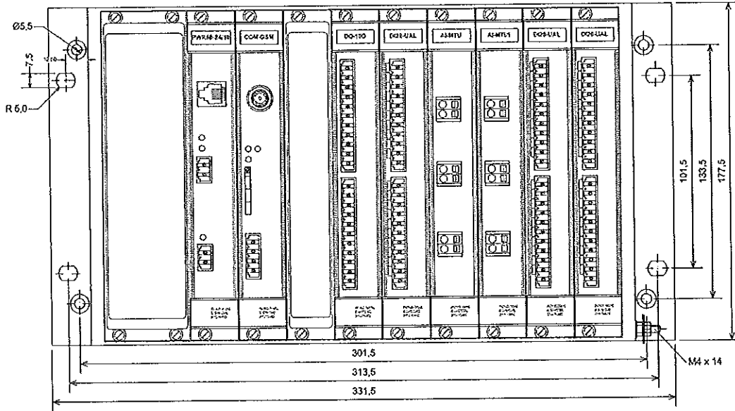
Dimensions of chassis with 10 slots
