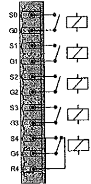
Outputs connection
