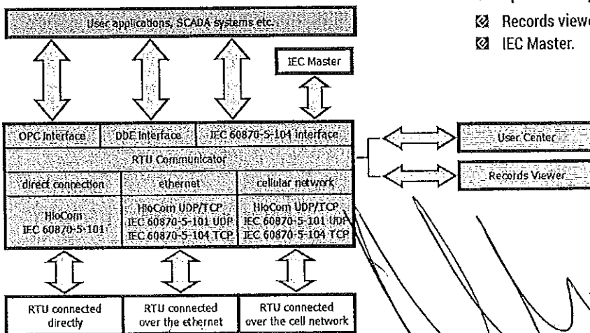
Communication scheme
