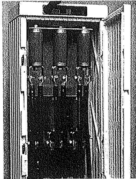
CPA arresters installed in a cubicle to protect HV cable sheath cross bonds
