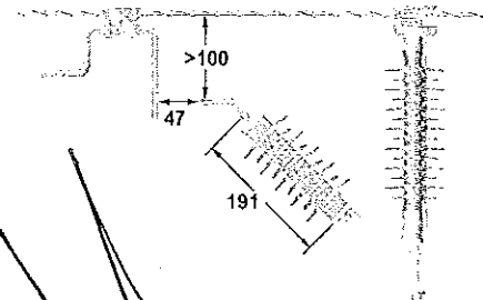
Typical Setup for U m 12 kV
