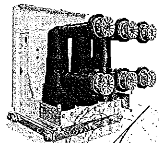
VD4 with poles in polyamide
