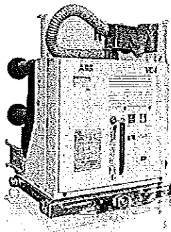
VD4 with poles in polyamide
